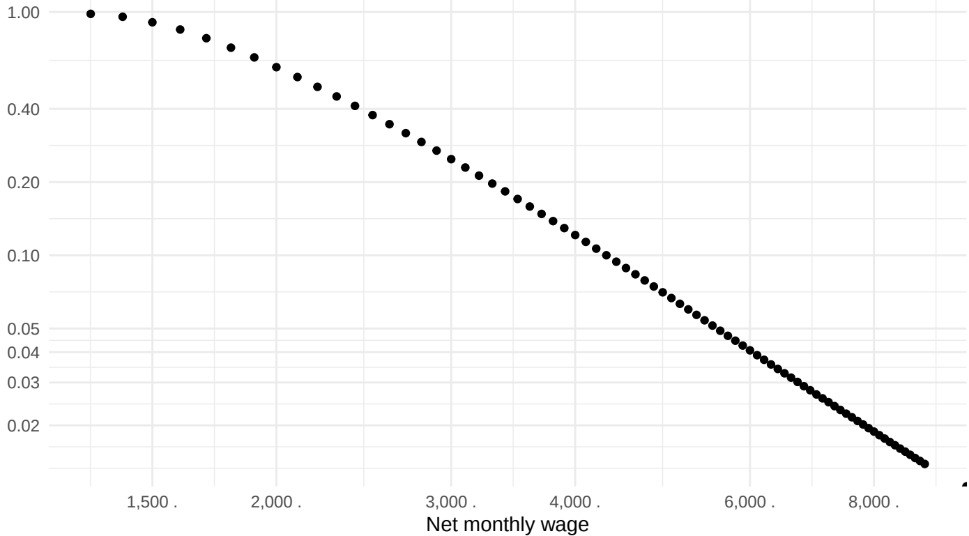
Countercumulative Distribution Function
